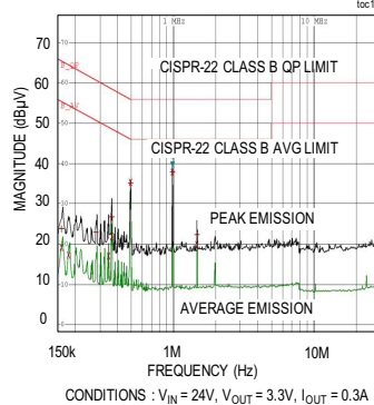
CONDUCTED EMISSION PLOT (EMI FILTER: C6, C7 = 0.1μF, C8 = 0.47μF, L1 = 82μH, C9 = 1μF)
