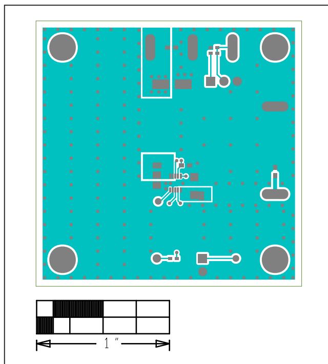
MAXM15463 EV Kit PCB Layout—Top Layer
