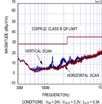
RADIATED EMISSION PLOT (C6 = 0.1μF, C7, C8, C9 = OPEN, L1 = SHORT)
