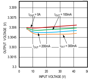
OUTPUT VOLTAGE vs. INPUT VOLTAGE V_{OUT} = 3.3V , PWM MODE
