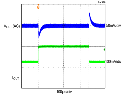
LOAD TRANSIENT RESPONSE V_{IN} = 24V , V_{OUT} = 3.3V , PWM MODE (LOAD CURRENT STEPPED FROM 150mA TO 300mA)
