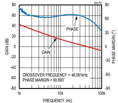
BODE PLOT V_{IN} = 24V , V_{OUT} = 3.3V , FULL LOAD, PWM MODE
