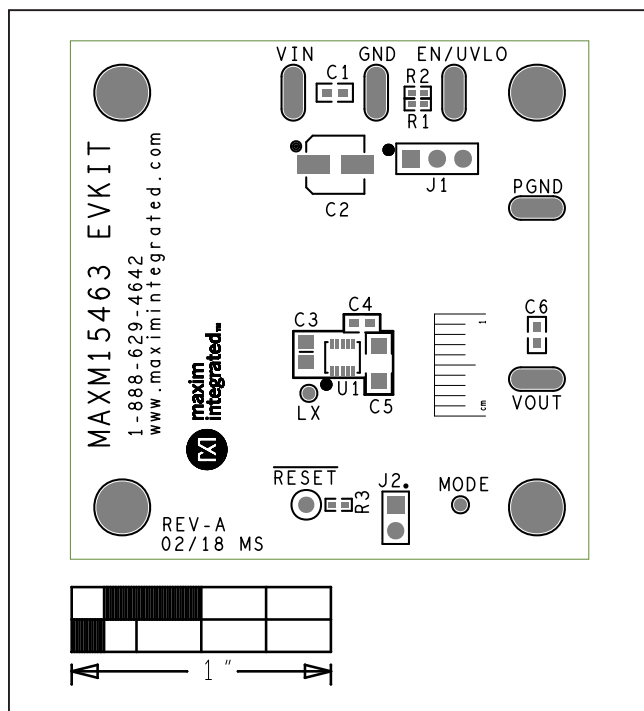
MAXM15463 EV Kit PCB Layout—Silk Top
