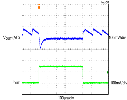
LOAD TRANSIENT RESPONSE V_{IN} = 24V , V_{OUT} = 3.3V , PFM MODE (LOAD CURRENT STEPPED FROM 5mA TO 150mA)
