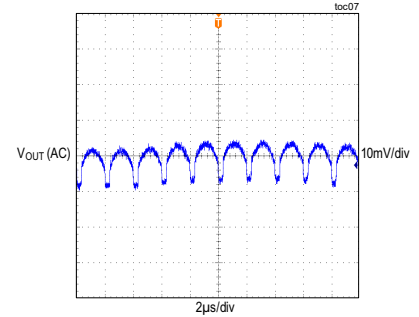
OUTPUT VOLTAGE RIPPLE V_{IN} = 24V , V_{OUT} = 3.3V , FULL LOAD, PWM MODE
